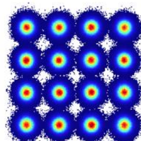
140 GBd 16QAM – 1.12 TBit/s EVM 9.5%
